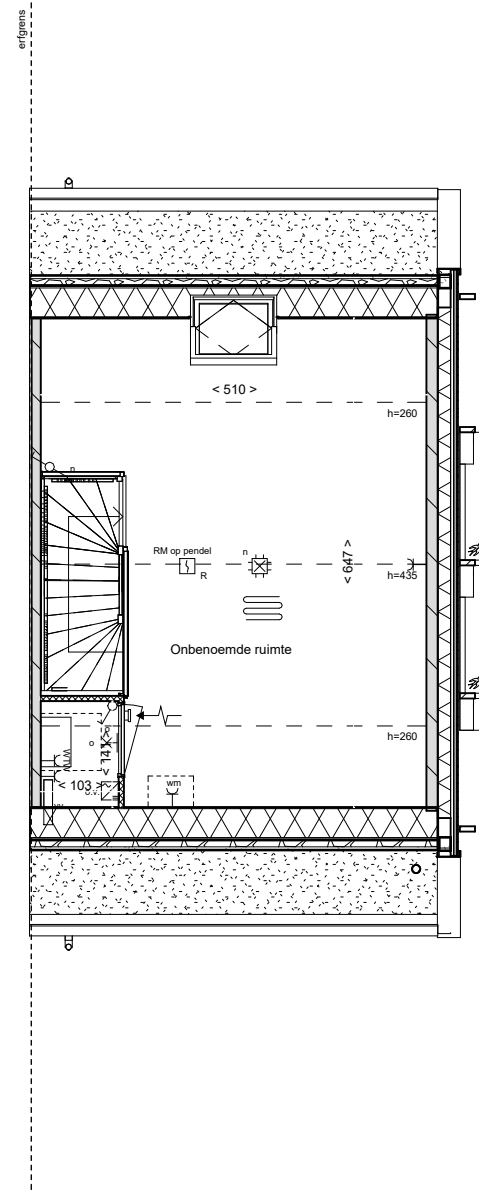
zolder
