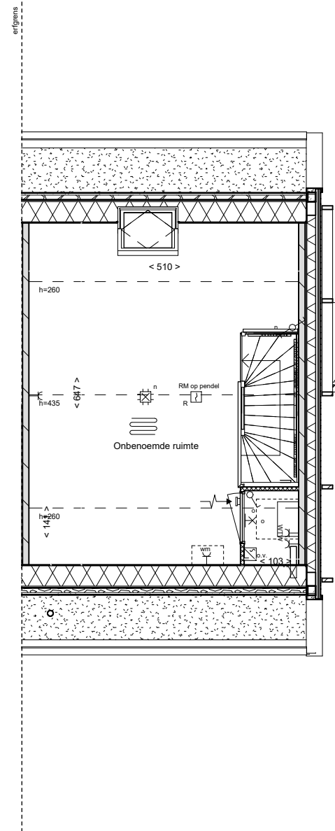
zolder
