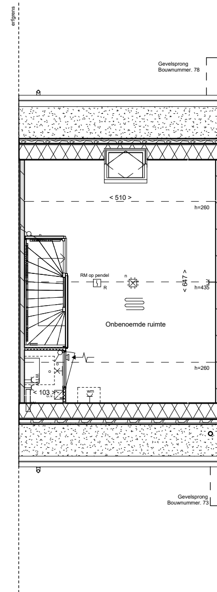
zolder
